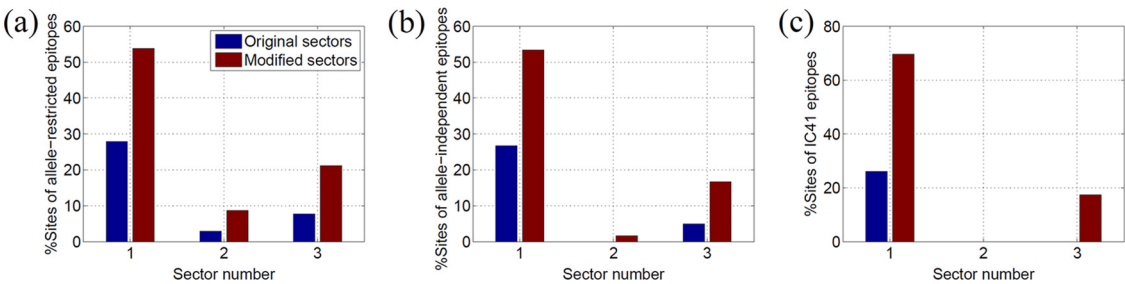
FIG A4 Analysis of the three sectors of NS3 constructed using the ICA method. (a) Percentage of sites in the NS3-specific allele-restricted protective epitopes present in the original sectors and the modified sectors obtained by incorporating the neighboring 100% conserved sites. (b) Percentage of sites in the NS3-specific allele-independent protective epitopes present in the original sectors and the modified sectors. (c) Percentage of sites in the NS3-specific IC41 epitopes present in the original sectors and the modified sectors.
