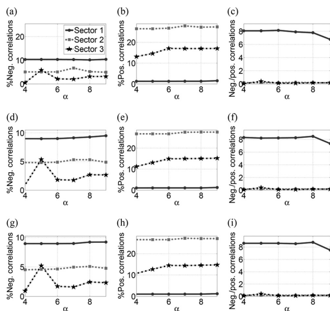
FIG A1 Consistency in the statistics of the three sectors of NS3 when the cleaned correlation matrix was constructed using selective large eigenvalues ( 4 < \alpha < 9 ). (a) The percentage of negative correlations. (b) The percentage of positive correlations. (c) The ratio of negative to positive correlations. (d to f) Statistics of the sectors as a function of the number of eigenvalues selected to construct the cleaned correlation matrix for NS3 using the RMT-based modified eigenvalue clipping method (43). (g to i) RMT-based estimation of true eigenvalues from sample eigenvalues (44).
