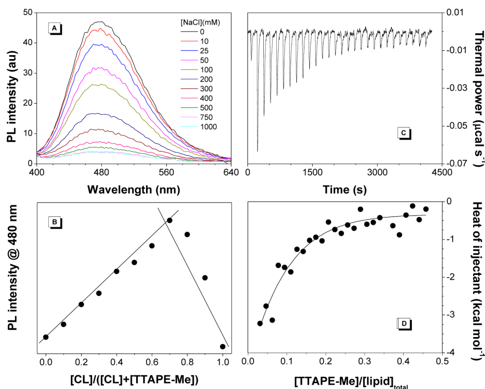
Figure 3. (A) Emission spectra of TTAPE-Me with CL-containing vesicles in the presence of varying concentrations of NaCl. [\text{dye}] = 10 \mu\text{M} ; [\text{lipid}]_{\text{total}} = 22 \mu\text{M} ; \lambda_{\text{ex}} = 350 \text{ nm} . (B) Job plot for determination of the binding stoichiometry of TTAPE-Me to CL-containing vesicles. The total concentration of TTAPE-Me and CL is kept at 20 \mu\text{M} . (C) Calorimetric curves at 25^\circ\text{C} for titration of CL-containing vesicles with serial injections of TTAPE-Me. (D) Binding isotherm as a function of [\text{TTAPE-Me}]/[\text{lipid}]_{\text{total}} molar ratio. CL-containing vesicles are composed of TOCL and DOPC (1:1 molar ratio).
