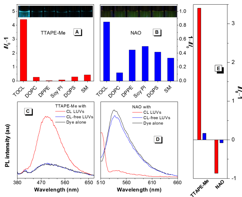
Figure 4. (A and B) Change in fluorescence intensity of (A) TTAPE-Me and (B) NAO with vesicles of different lipid contents (left to right: 20% TOCL, 100% DOPC, 40% DPPE, 2% soy PI, 1% DOPS, and 2% SM; the rest of each type of vesicle is filled by DOPC). Insets: Corresponding fluorescence photographs of TTAPE-Me and NAO solutions in the presence of these LUVs. (C and D) Emission spectra of (C) TTAPE-Me and (D) NAO with CL-containing and CL-free all-component vesicles. (E) Bar chart of the change in fluorescence intensity shown in panels C and D (red, CL-containing vesicles; blue, CL-free vesicles). [dye] = 10 \mu M; [lipid] total = 22 \mu M; for TTAPE-Me, \lambda_{\text{ex}} = 350 nm, \lambda_{\text{em}} = 480 nm; for NAO, \lambda_{\text{ex}} = 499 nm, \lambda_{\text{em}} = 530 nm.
