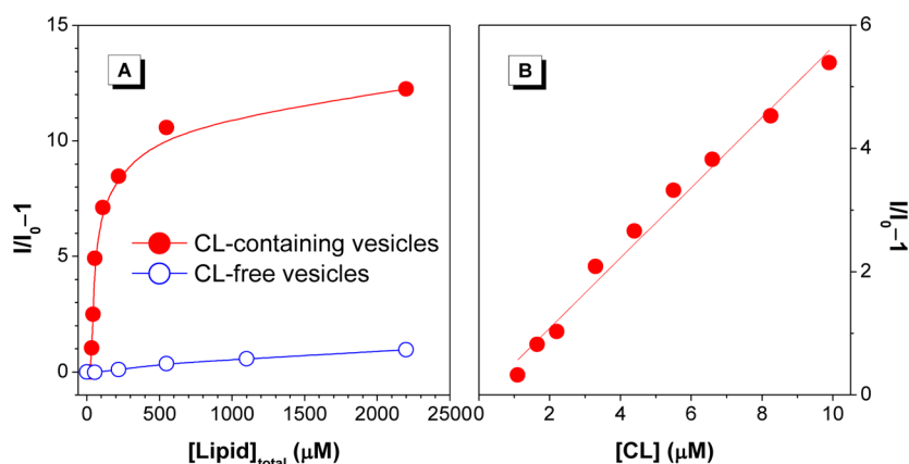
Figure 2. (A) Plot of the fluorescence enhancement ( I/I_0 - 1 ) of TTAPE-Me at 480 nm with CL-containing and CL-free vesicles. (B) Linear region of the I/I_0 - 1 value vs CL concentration. [\text{dye}] = 10 \mu\text{M} ; \lambda_{\text{ex}} = 350 \text{ nm} .
