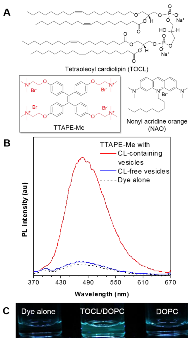
Figure 1. (A) Chemical structures of TOCL, TTAPE-Me, and NAO. (B) Emission spectra and (C) the corresponding fluorescence photographs of TTAPE-Me solutions in the absence and presence of vesicles, with and without CL. CL-containing and CL-free vesicles are composed of TOCL/DOPC (1:1 molar ratio, CL-containing) and pure DOPC (CL-free), respectively, in a 25 mM HEPES buffer at pH 7.4. [dye] = 10 \mu M; [lipid] total = 22 \mu M; \lambda_{\text{ex}} = 350 nm.
