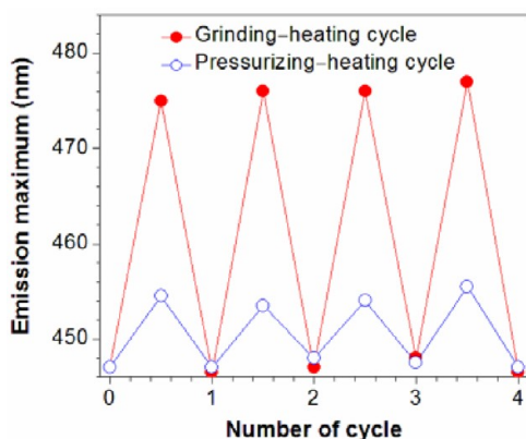
Figure 8. Reversible switching of emission of ( E )-BPHTATPE by repeated grinding–heating (red line) or pressurization–heating (blue line) cycle; heating: 120 °C, 1 min; pressurization: 30 MPa, 1 min; \lambda_{\text{ex}} = 332 nm.
