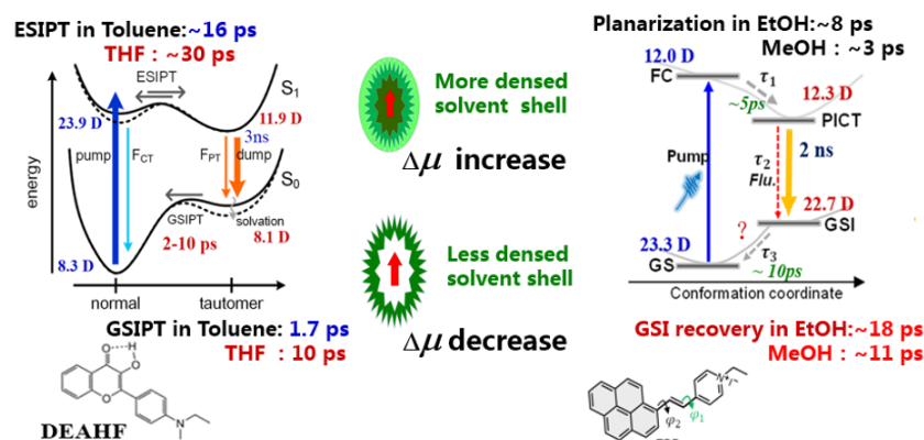
Figure 1. Solvation-dependent excited state evolution during the intrinsic photocycle upon state-by-state dipole moment changes.
